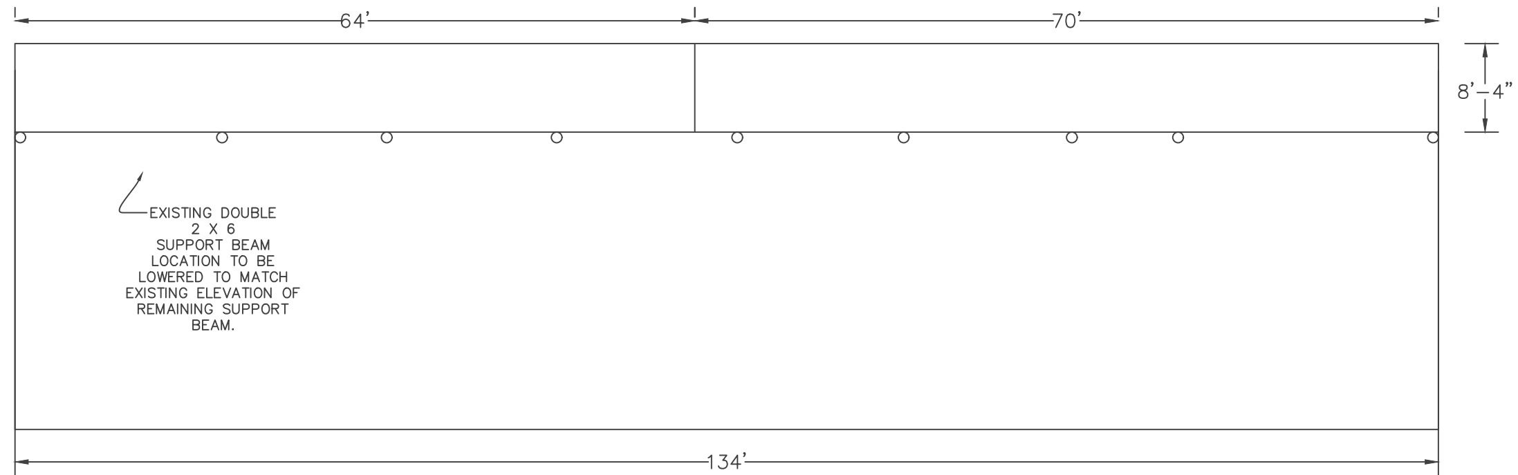
CANOPY LAYOUT
