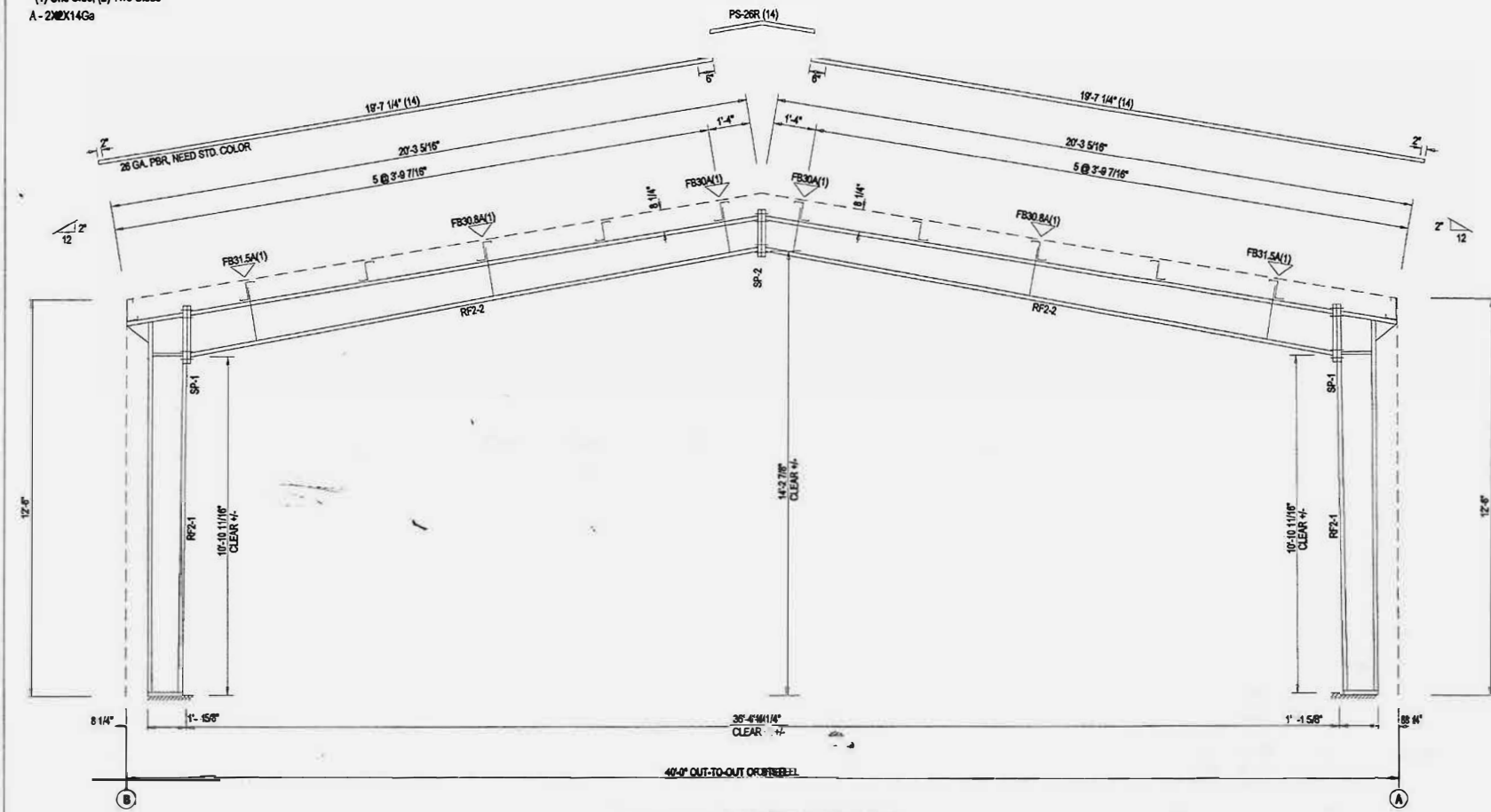
RIGID FRAME ELEVATION: FRAME LINE 2
